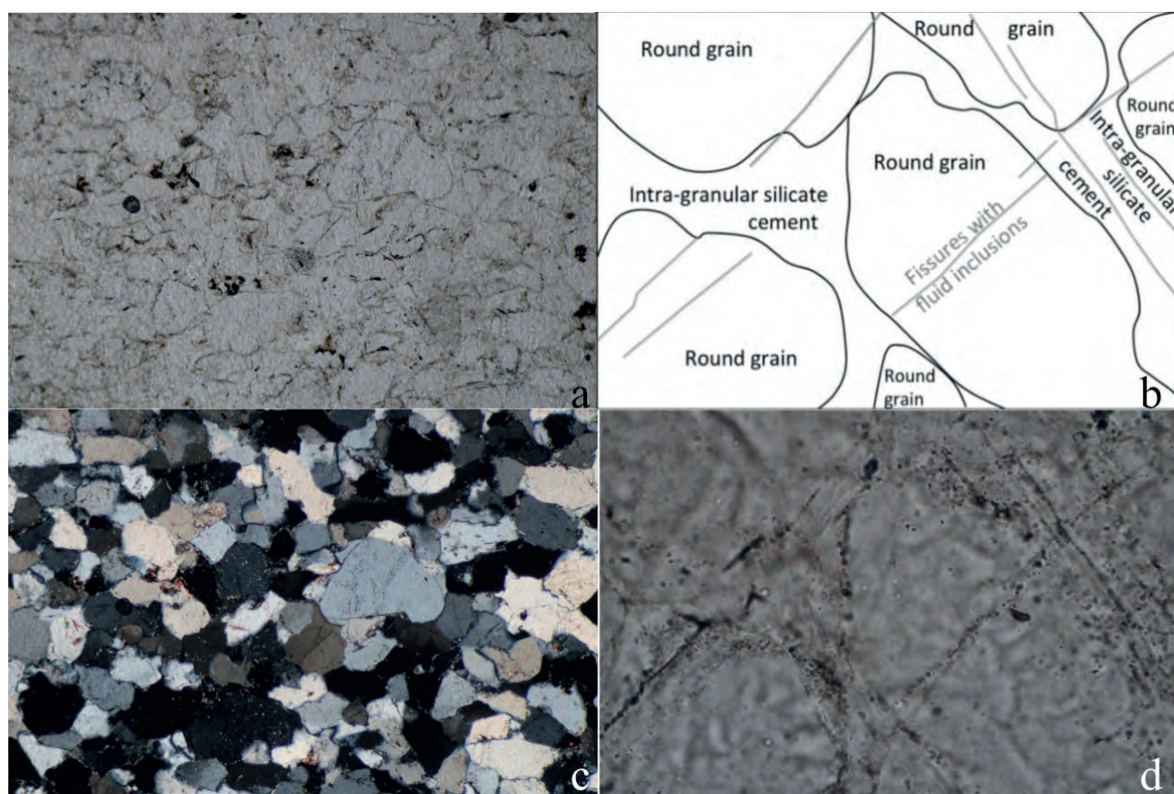
Figure 10. Microphotographs showing the petrographic characteristics of samples Es 11 a. and c. Quartz-sandstone Es 11 composed of sub-rounded quartz grains and sub-angular feldspar crystals, whose porosity is filled by intergranular and intersertal silica cement, indicating a moderate degree of maturity. There are detrital muscovite crystals or included in quartz, and hematite filling some pores (figure length 5,5 mm, 50x magnification). b. and d. Detail of Es 10: rounded quartz grains between which an intra-granular silicate cement crystallizes, indicating a high diagenetic degree (mesogenesis) (figure length 0,25 mm, 800x magnification). (Microphotographs. R. Ferreiro Máhlmann).
