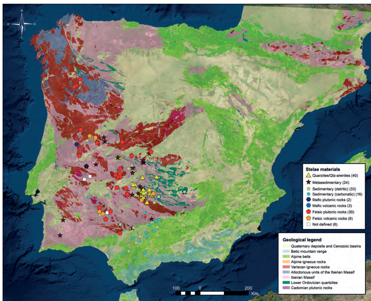
Figure 1. Simplified geological map of the Iberian Peninsula with legend, showing FBA-EIA stelae with their generalized lithotypes (Map: E. Merino-Martínez).
