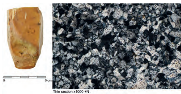
Figure 5. A. Quartzite tool (Po 22) (Foto: M. Kinsky). B. Diablastic microstructure (Microphotograph: R. Ferreiro Mählmann).
