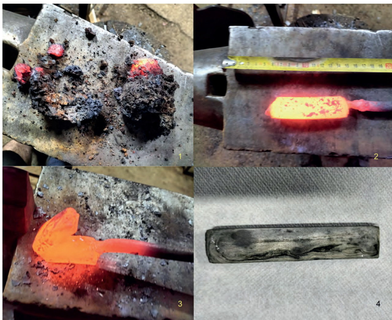
Figure 12. (1) Transformation from pieces of the bloom through (2) refining and (3) welding to (4) a piece of refined steel, etched to reveal the different carbon (the darker, the higher) contents in the welded layers, with some slag inclusions (Fotos: T. Mink).
