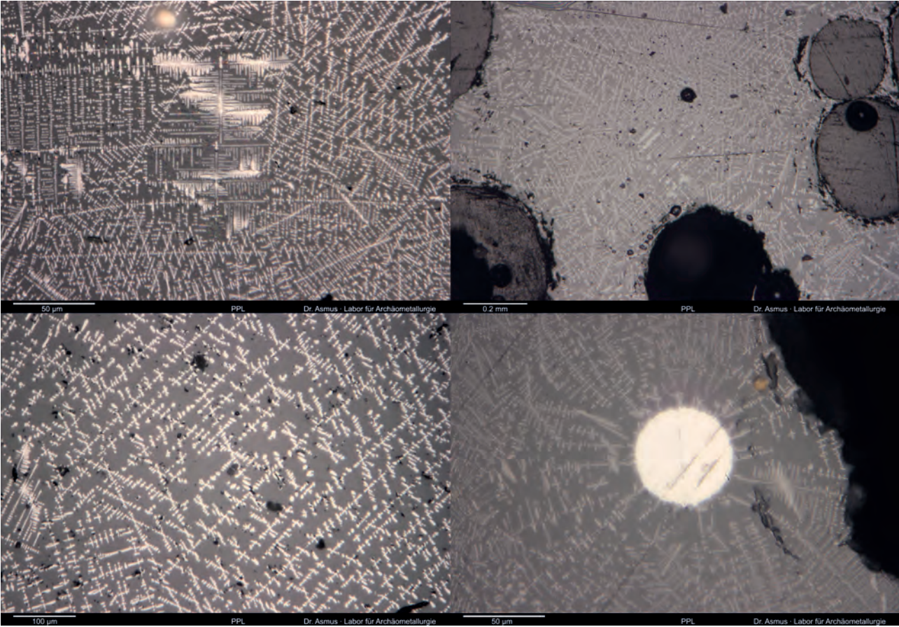
Figure 3: These are typical section for the five tapping events. Top left 1. tapping, there is only wüstite as discernable phase present, the matrix is either fine sub-microscopical fayalite, or a glass with near fayalitic composition. Top right: slag of the second tapping event. It is very similar in its composition. Bottom left is from the fourth tapping event and matches the slag from the third tapping event: This is wüstite in glass and/or sub-microscopical fayalite. Bottom left: The final tapping before retrieving the bloom. It is also very similar in it composition as well in its grain sizes. Image: © B. Asmus.
