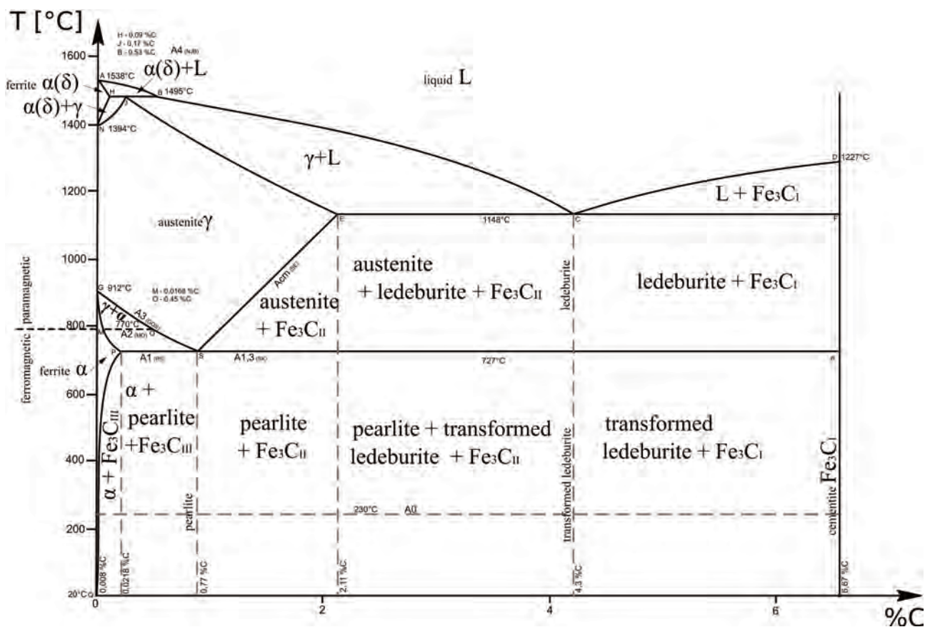
Figure 5: The iron carbon phase diagram is used to map and understand the phase transformations in this alloy. It is for equilibrium states only, so it cannot inform us on heat treatment processes.
