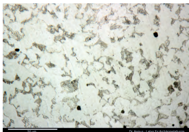
Figure 21: Steel chisel from Rocha do Vigio, etched 2% Nital. This area consists mostly of ferrite grains and some pearlite nodules. This represents the areas with the lowest carbon content of the chisel. Image: © B. Asmus.
