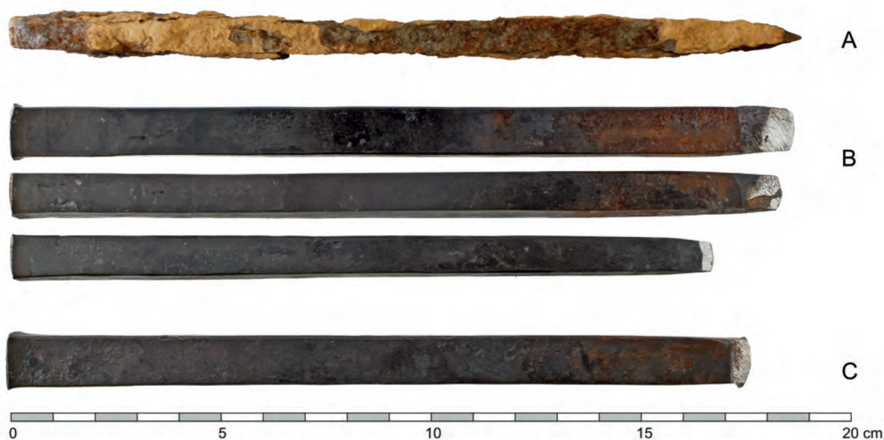
Figure 9. A. Chisel from Rocha do Vigio (Foto: R. Araque). B. Hardened, quenched and tempered C60 steel chisel replications by Alexander Richter, Fragua Fuirio, Seville. C. Unhardened, soft annealed C60 steel chisel replication with deformed blade after use on silicate quartz arenite (Fotos: M. Kinsky).
