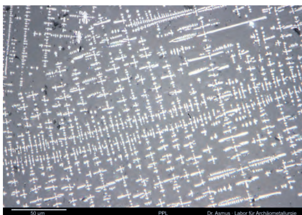
Figure 2: The image width is 275 \mu\text{m} , PPL. Third tapping event. It shows a typical section of the slag at high magnification. The only discernable phase is wüstite (white), the grey matrix is either a glass of fayalitic composition or submicroscopic fayalite. Image: © B. Asmus.
