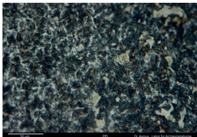
Figure 7: Etched 2% Nital. Image width 275 \mu\text{m} . Higher magnification of a region with an almost pure pearlitic composition, i.e. very close to the eutectoid point of 0.77 mass% carbon. Image: © B. Asmus.
