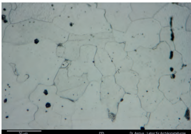
Figure 16: Heat treated sample, etched 2% Nital. More or less pure ferrite. The critical cooling rate was exceeded, otherwise there would be no ferrite. Image: © B. Asmus.
