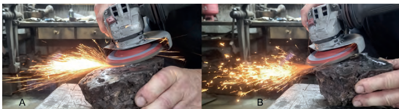
Figure 11. Spark test by cutting a bloom with a high carbon content, which renders it hardenable. There are plentiful starry sparks that open quickly (Foto: T. Mink).
