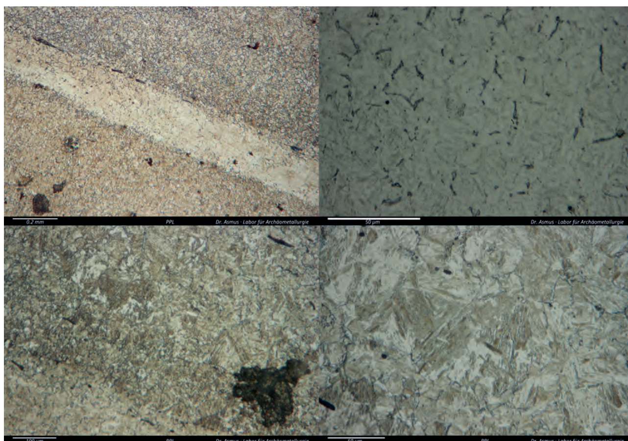
Figure 19: The second heat treated sample. It shows martensite, as predicted from the CCT diagram. Etched with Nital 2%. PPL. Top left: Overview of various martensitic structures. The lightly coloured area is a layer of ferrite with a very low carbon content. Top right: Even the mostly ferritic areas underwent martensitic transformation. Bottom left: Martensite in an area of the sample with carbon content of about 0.3 mass% C. Bottom right: Lath martensite at higher magnification. Image: © B. Asmus.
