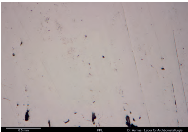
Figure 9: Image width: 2.7 mm. PPL. The section shows a polished section of unrefined bloom. There are a few small slag inclusions. Porosity at the bottom is along incompletely fused iron grains. Image: © B. Asmus.
