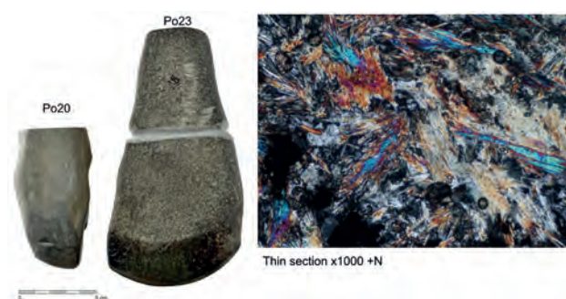
Figure 6. A. Actinolite skarn tools (Po 20 and Po 23) (Foto: M. Kinsky). B. Fibroblastic, diablastic microstructure of Po 20 (Microphotograph: R. Ferreiro Mählmann).
