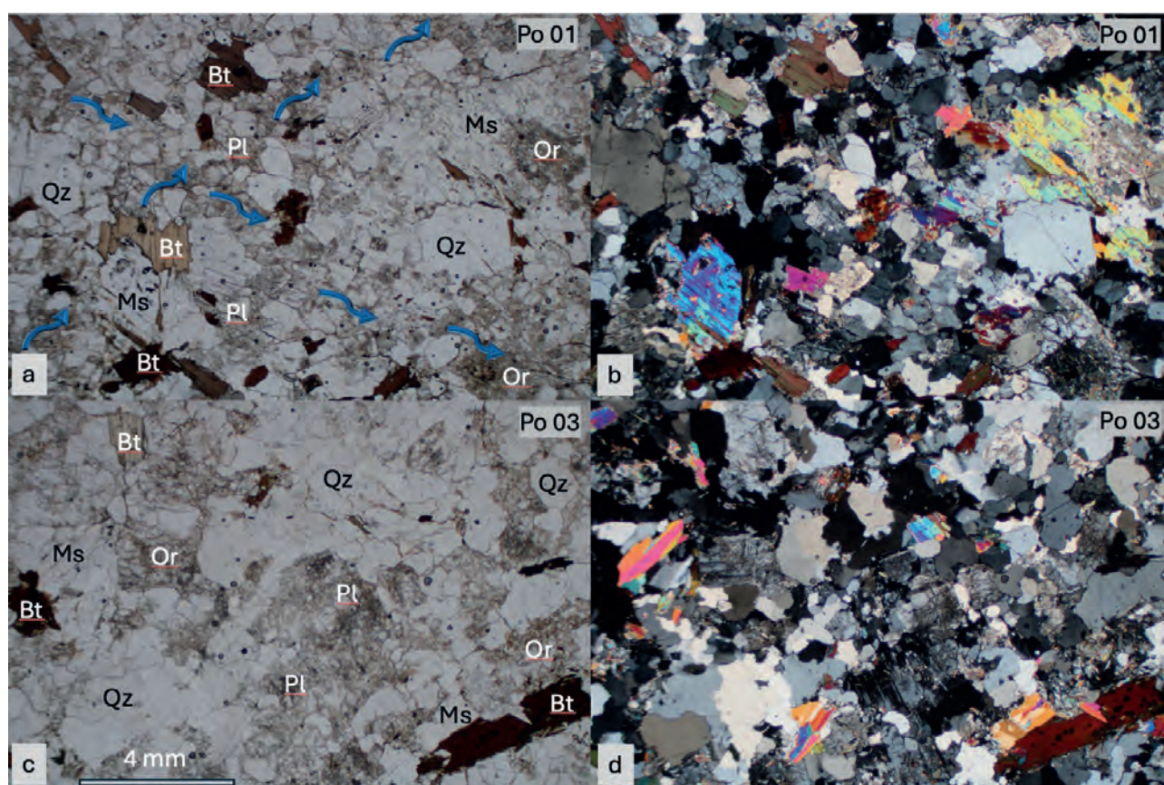
Figure 4. Baraçal 1 (Po 01) and Cabeço do Cornelho aplite (Po 03): Microphotographs with plane polarized (a and c) and crossed polarized light (b and d) (magnification: 16 x). In a. and c. feldspar (Pl = plagioclase, Or = orthoclase) can be easily recognized by the sericitized rough surface and distinguished from the colorless quartz (Qz) and muscovite (Ms). Biotite (Bt) shows an intensive pleochroism from light brown to dark red/isotropic (black). The blue wavy arrows indicate the direction of fluid alteration affecting mostly the feldspars, but also Bt (center of figure a, green alteration). (Microphotographs. R. Ferreira Máhlmann).
