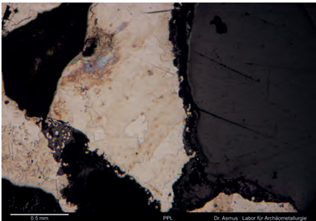
Figure 10: Polished section of bloom. Hardly slag inclusions. Only partly fused along the grain boundaries, this section display this a elongated pores at the bottom. Image: © B. Asmus.
