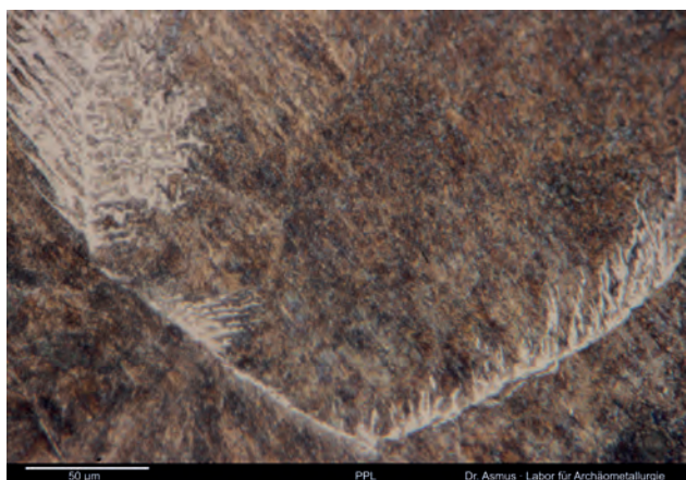
Figure 12: Bloom, Widmanstätten ferrite, is found throughout the heterogeneous sample, making this a low carbon steel. These structures do not develop near the eutectoid point. Image: © B. Asmus.
