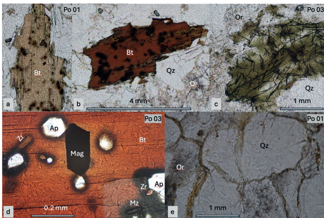
Figure 5. Baraçal 1 (Po 01) and Cabeço do Cornelho aplite (Po 03): Microphotographs with plane polarized light. Figure a. and b. have the same size (50 x) and show biotite (Bt) with an intensive pleochroism from light brown to dark red/isotropic (black). In figure c. a green altered biotite (see Figure 4a. at the center) is transformed to chlorite with a rutile needle sagenite microstructure (100 x). In d. all inclusions, except magnetite (Mag) cause pleochroic halos (Ap = apatite, Mz = monazite, Zr = zircon, 2000 x). In e. limonite in grain contacts around quartz (Qz) and orthoclase (Or) fills the space in the fissures lowering the cohesion (100 x). If Po 01 is indicated the same can be observed in Po 03 and vice versa. (Microphotographs. R. Ferreiro Mählmann).
