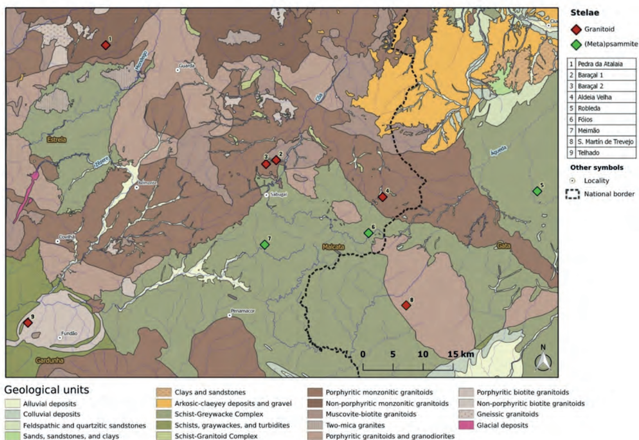
Fig. 3. Simplified geological map showing the location of western Iberian stelae around the Western Iberian Central System. (Map: M. Osório)
