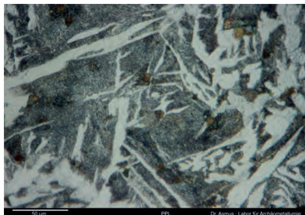
Figure 17: Heat treated experimental steel sample. Etched 2% Nital. The constituents are allotriomorphic ferrite, that grew along the former austenite grains, as well as fine grained pearlite and bainite. No martensite was encountered in the whole sample. Image: © B. Asmus.
