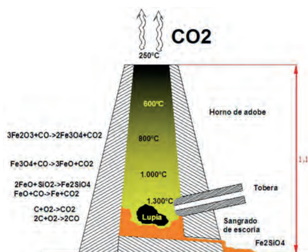
Figure 6. Schematic furnace and most common chemicals reactions (Drawing: T. Mink).
