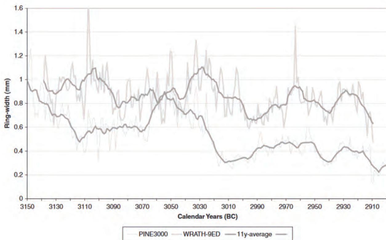
Figure 3: Ring-width plot of sequences WRATH-9ED (upper) and PINE3000 edited to span 3150–2900 BC (lower), which cross-match together with a t-value of 5.7. Similarities in the patterns of variation at both high and medium frequencies can be seen (after Moir et al. 2010, 10, Figure 5).
