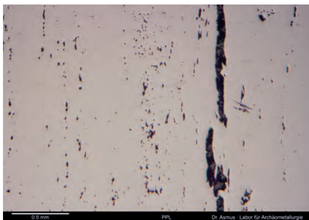
Figure 13: The layered structure of the steel is unmistakable. The slag stringers are aligned along the direction of the fire-welded areas. The structure has no improperly welded areas. Quite contrary to the bloom. Image: © B. Asmus.
