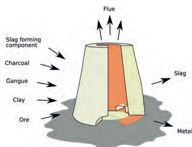
Figure 1: A schema of a smelting furnace, its educts, by-, waste and end products. Image: ©B. Asmus.
