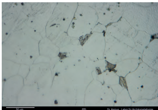
Figure 6: Etched 2% Nital. Image width 275 \mu\text{m} . Higher magnification of a region with very little carbon content. This is almost pure ferrite, situated towards the edges of the sample. Image: © B. Asmus.
